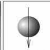
Measured photon is only in one state (spin = down).
